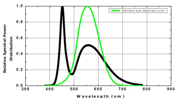
White LED Light Typical Spectrum
