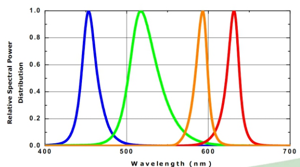
R/G/B LED Light Typical Spectrum
